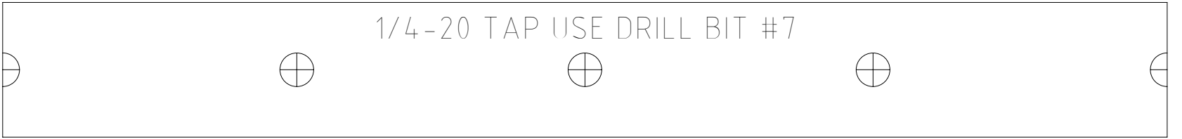
2" PVC COUPLING RETAINING BOLT TEMPLATE
